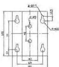
Mounting plate
