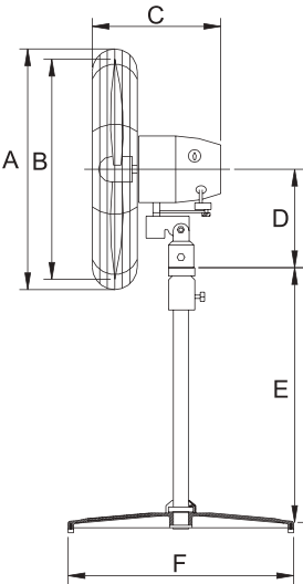
Outline dimensions
